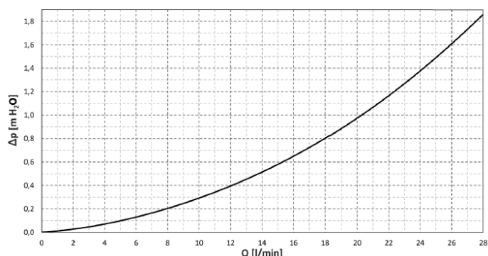
Connections G 1" M – code 20577
