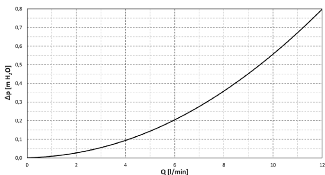
Connections G 3/4" M – code 20581
