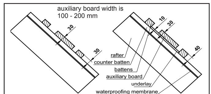
Fig. 3: Underlay to match thick battens
