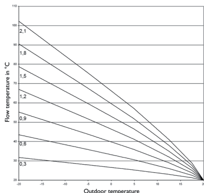
heating curves
