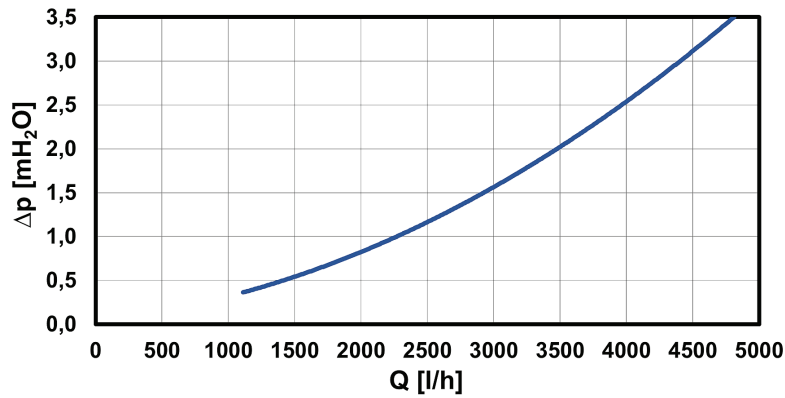
Pressure drop on the brine side
