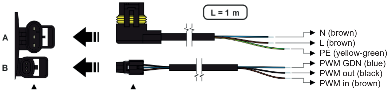
socket for power supply (A) and signal transmission (B) power supply (A) and signal (B) connectors
